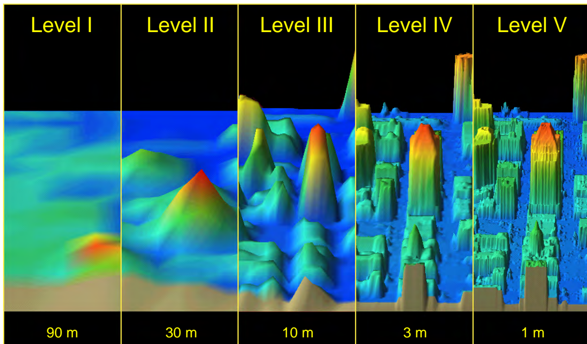
Figure 2. Visual depiction of the detail provided at five different spatial resolutions (Image courtesy of the Engineer Topographic Laboratories)
